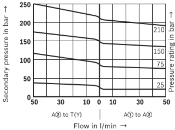
p_A - q_V characteristic curves – Version "A"
