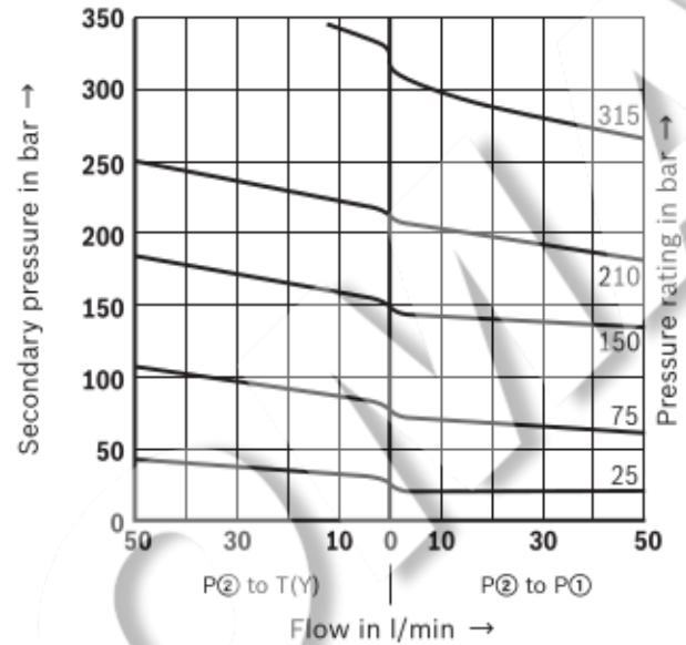
p_A - q_V characteristic curves – Version "B" and "P"
